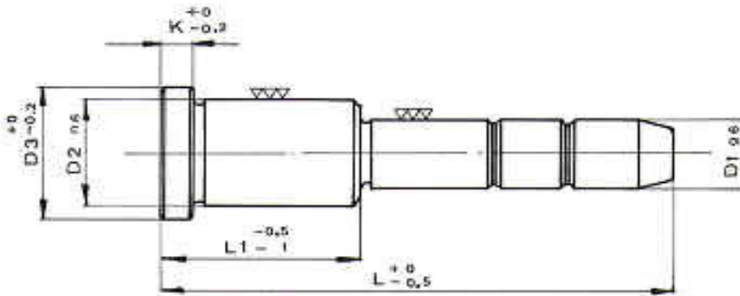
GUIDE PILLAR WITH TWO STEP Material Suj2, 1.2067, 16NiCr4 Hardness: HRC55-60
